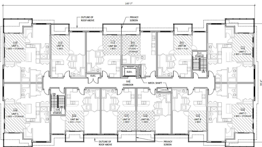
5th floor
