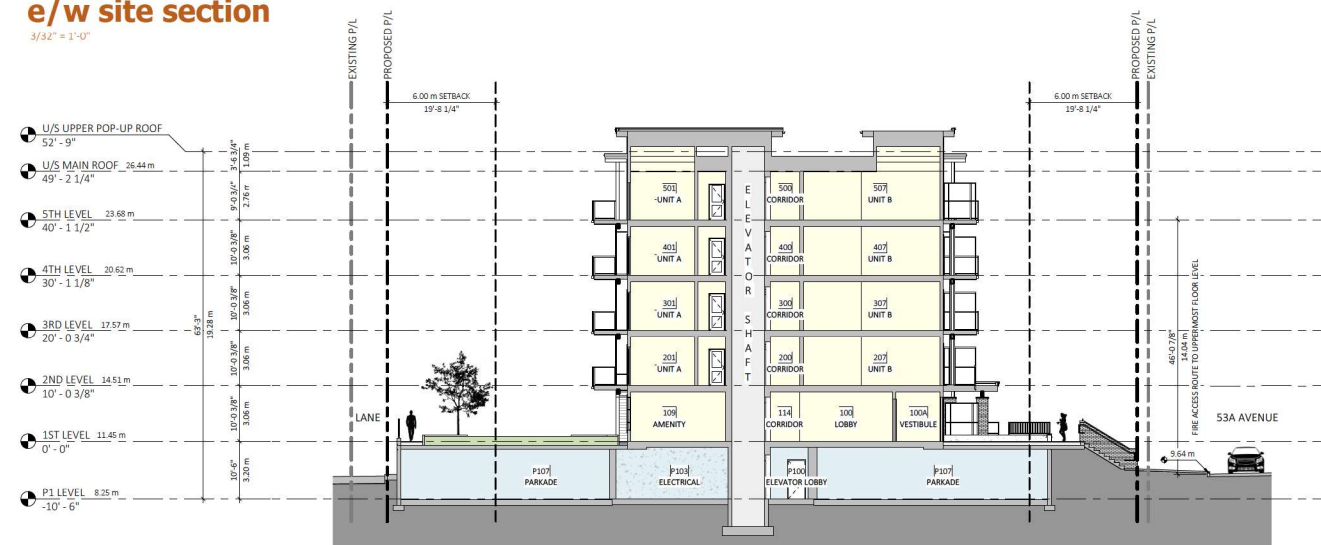
n/s site section 3/32" = 1'-0"
