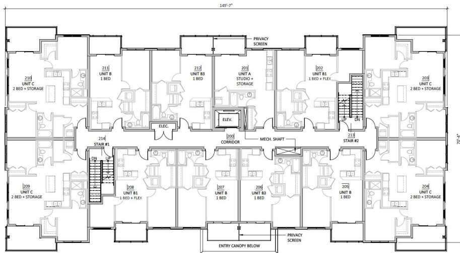
2nd floor
