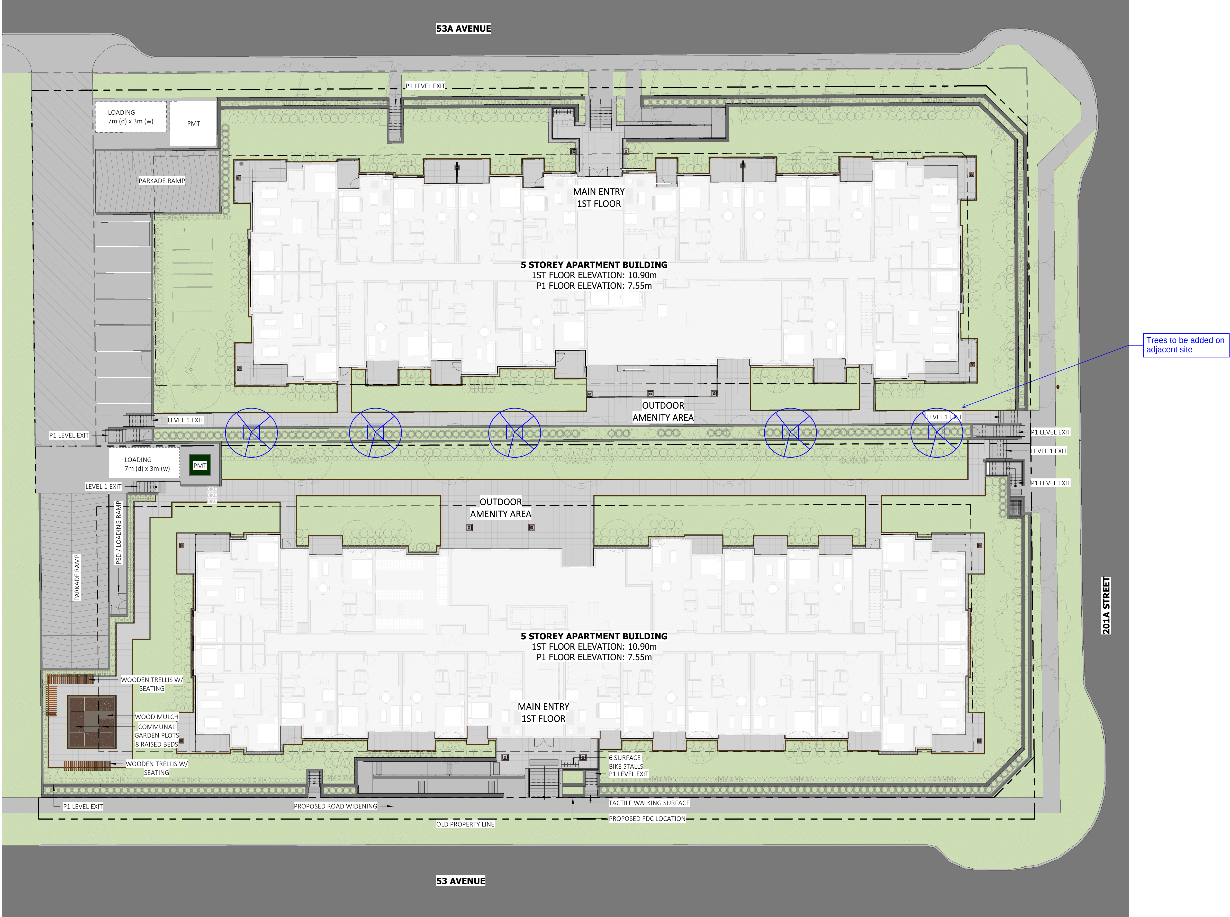
combined site plans 1/16" = 1'-0"
