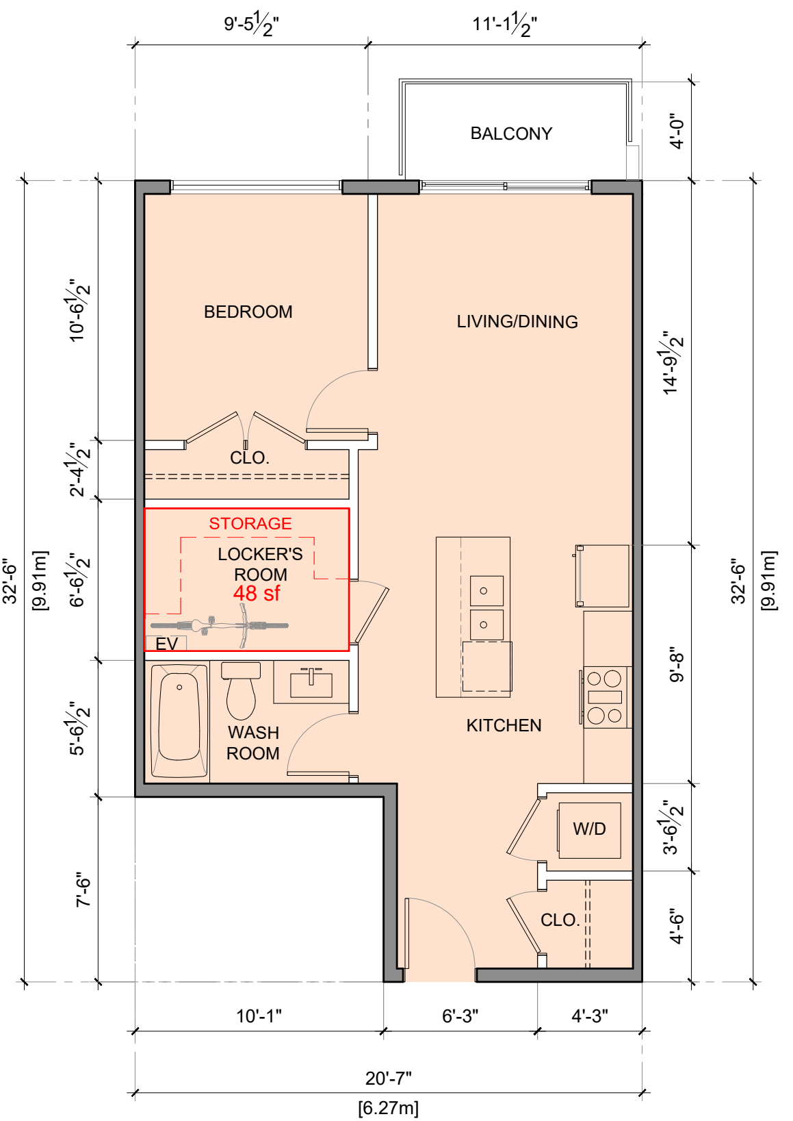
2 UNIT-G 3/16"=1'-0"
