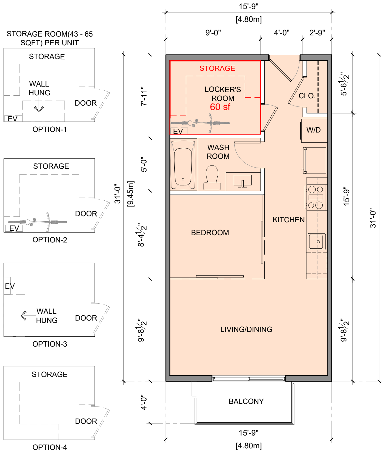
1 UNIT-C 3/16"=1'-0"
