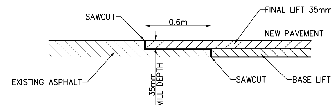
JOINT MILL AND OVERLAY DETAIL N.T.S.
